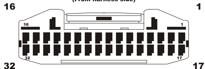
MAIN CONNECTOR (From harness side)
